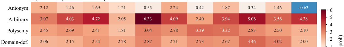
(b) Effect by prompt style
