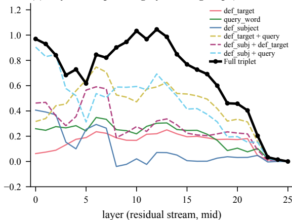
(a) Layer-wise patching by source group (Gemma-2-2B)
