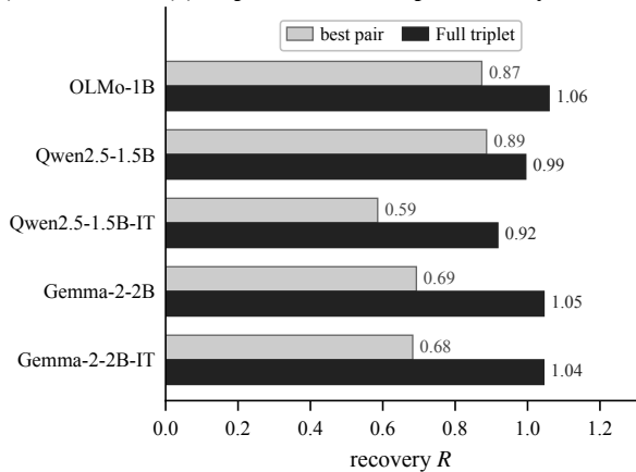
(b) Triplet exceeds best pair in every model
