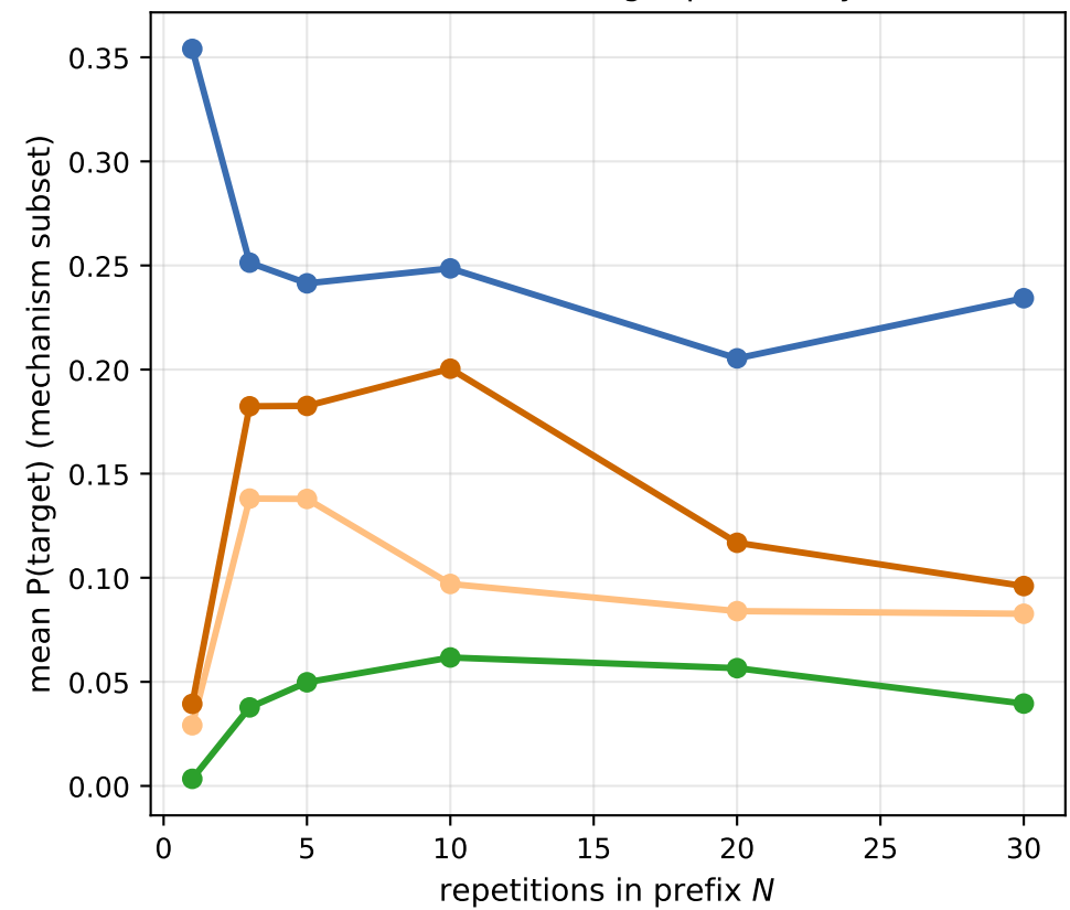
(c) Slot-state target probability
