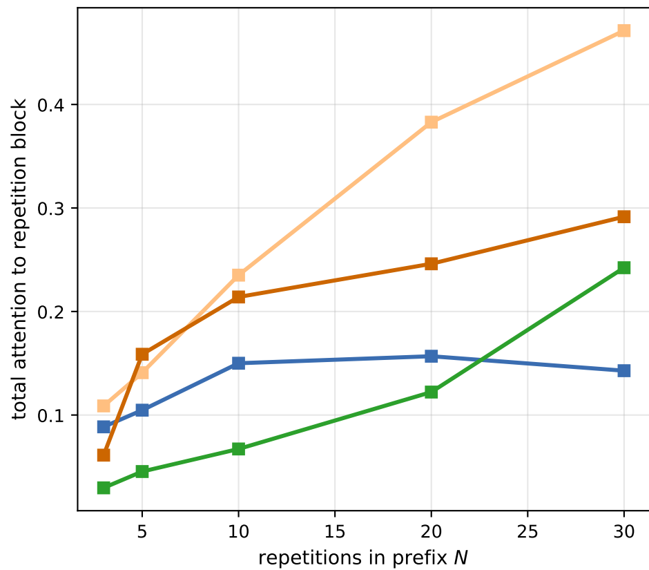
(b) Total block budget vs N
