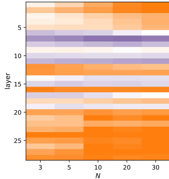
ModernBERT-large (MLM, 28 layers)
