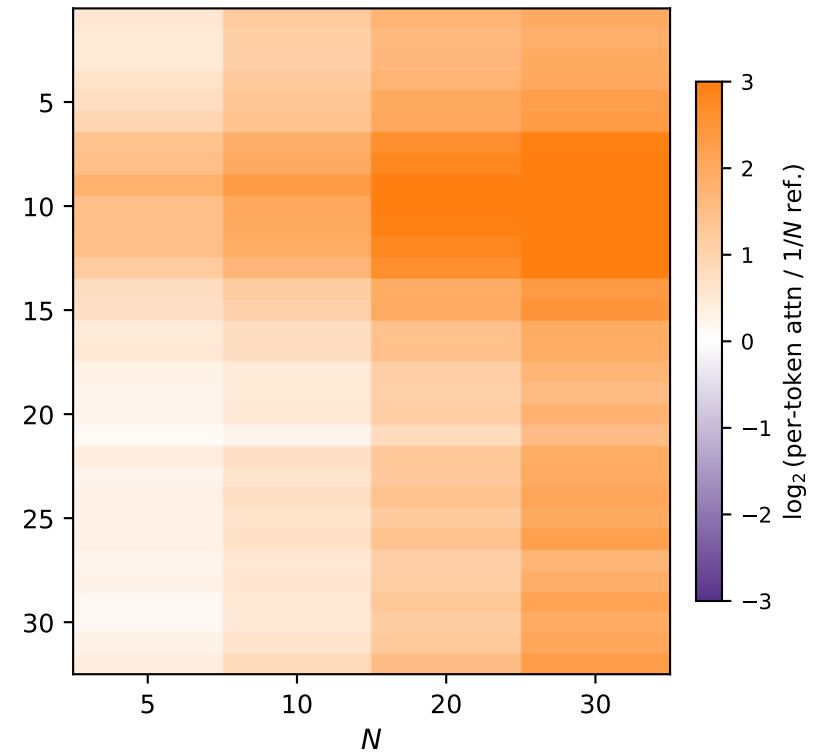
OLMo-2-7B (CLM, 32 layers)
