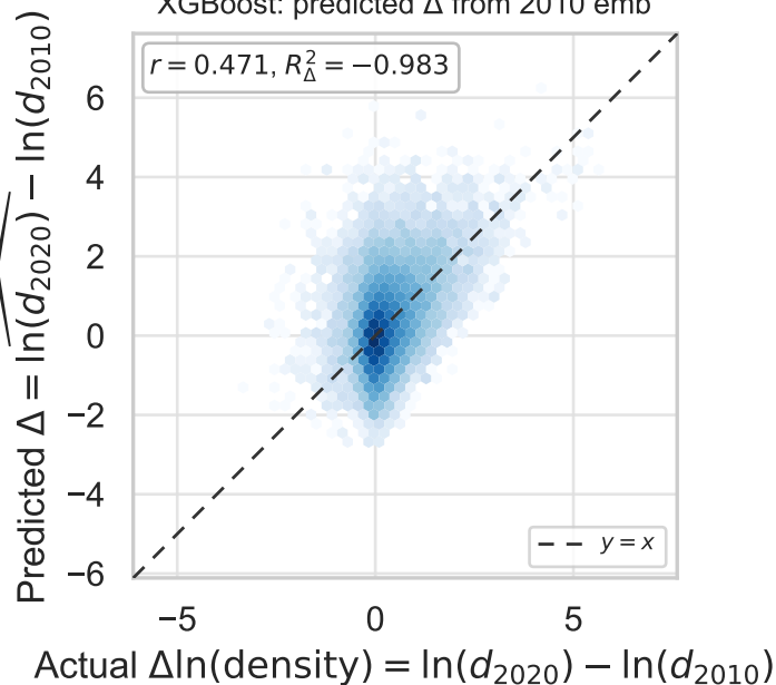
XGBoost: predicted \Delta from 2010 emb
