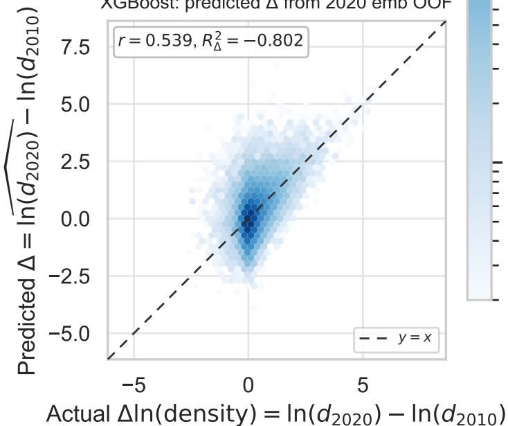
XGBoost: predicted \Delta from 2020 emb OOF
