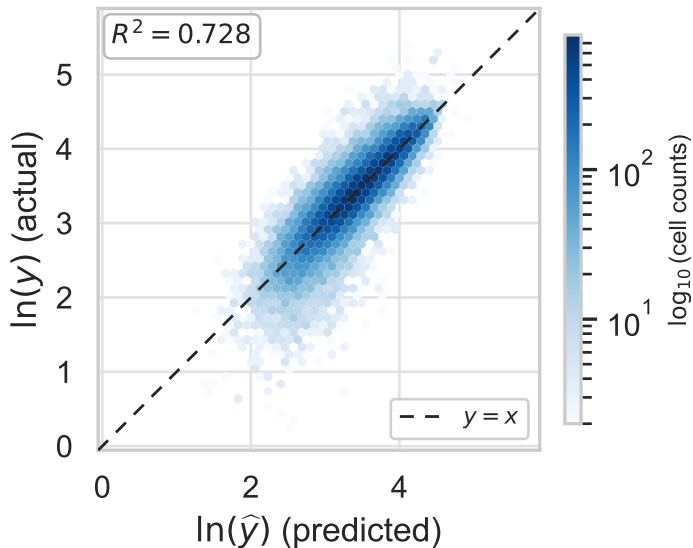
XGBoost
