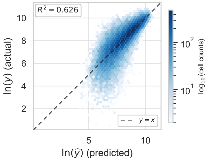
XGBoost
