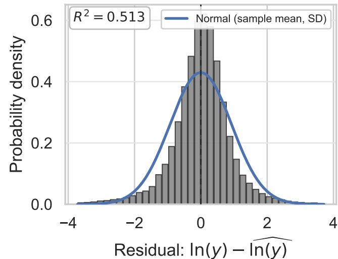
Ridge
