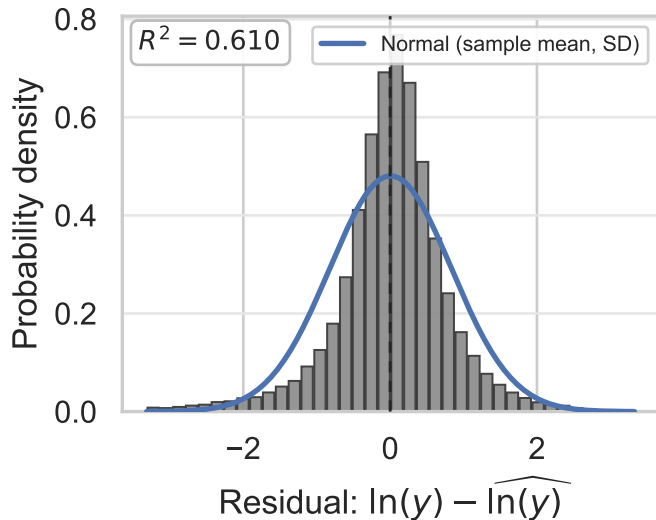
XGBoost
