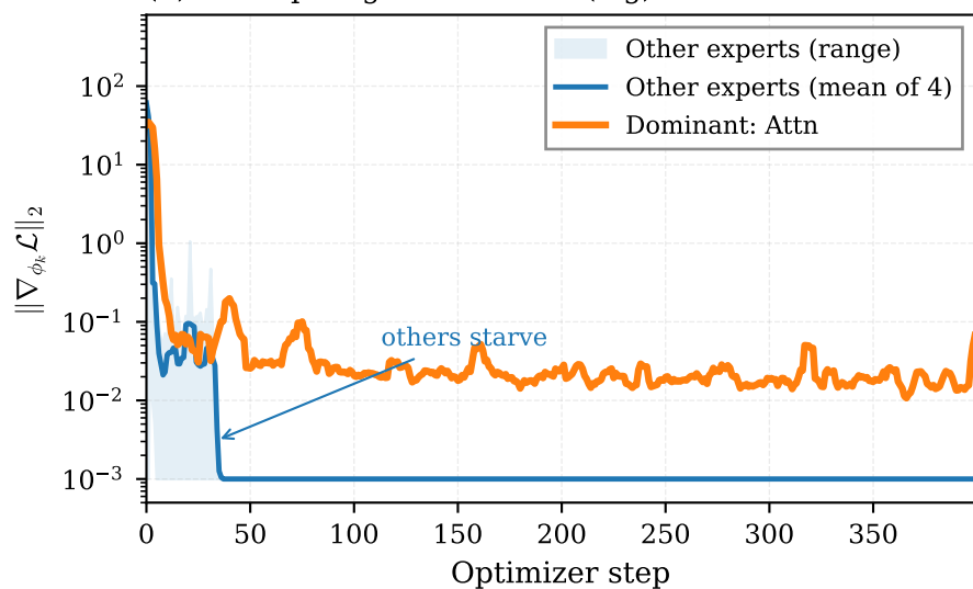
(b) Per-expert gradient norm (log)
