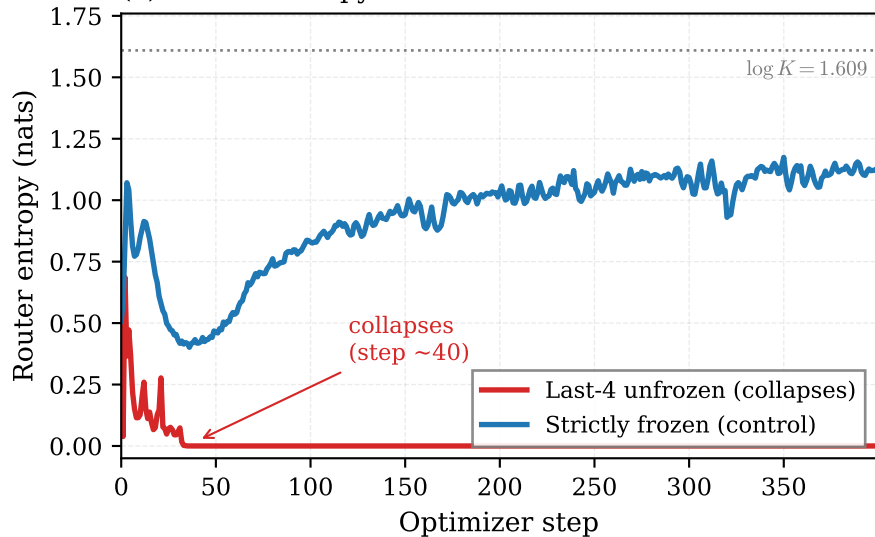
(a) Router entropy
