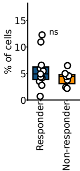
CD8_T
