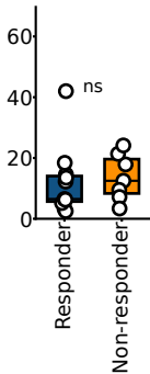
HSPC
