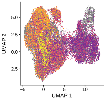
UMAP by Clonotype Frequency
