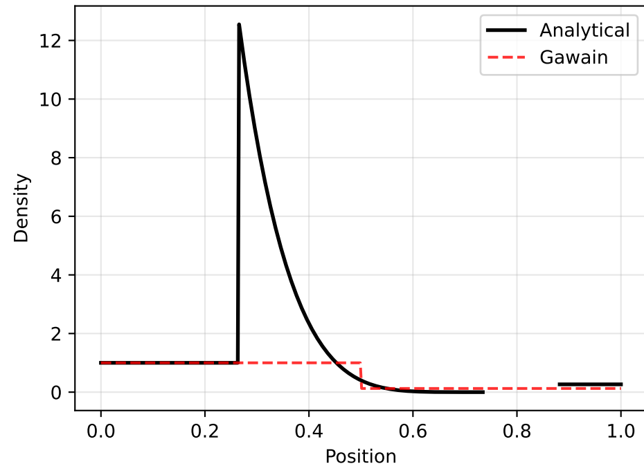
Sod Shock Tube: Density
