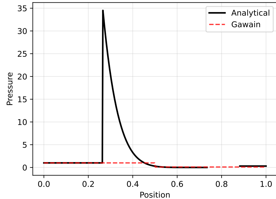
Sod Shock Tube: Pressure
