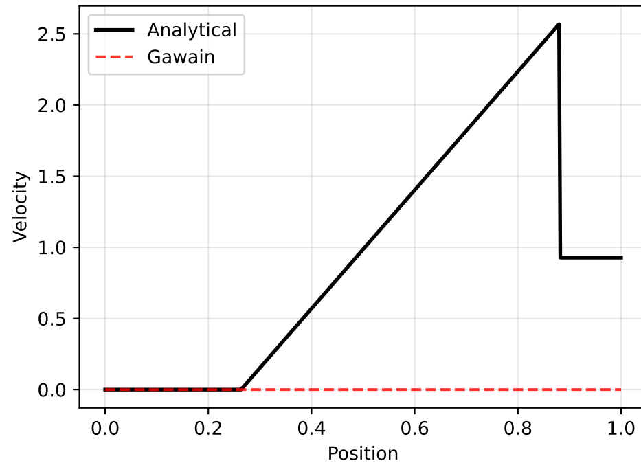
Sod Shock Tube: Velocity
