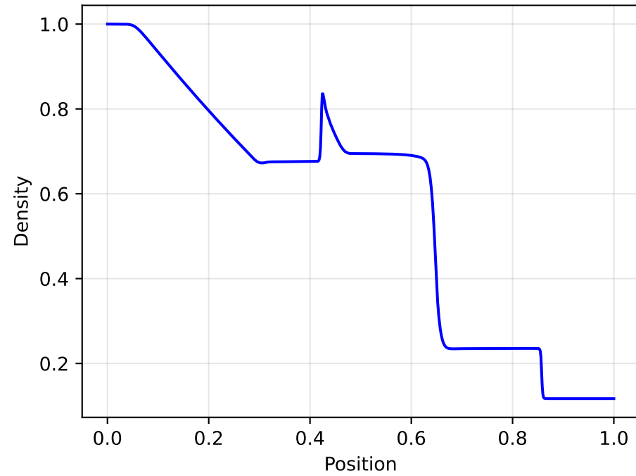
Brio-Wu MHD: Density
