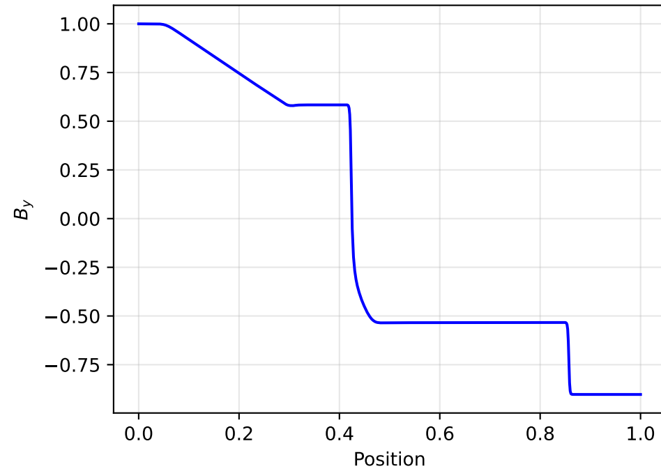
Brio-Wu MHD: Transverse Magnetic Field
