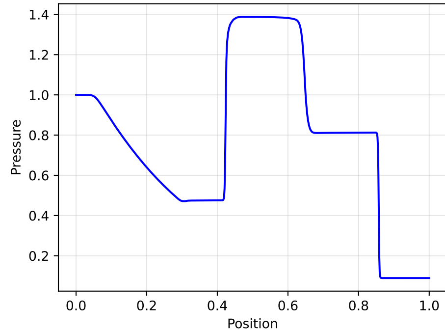
Brio-Wu MHD: Pressure
