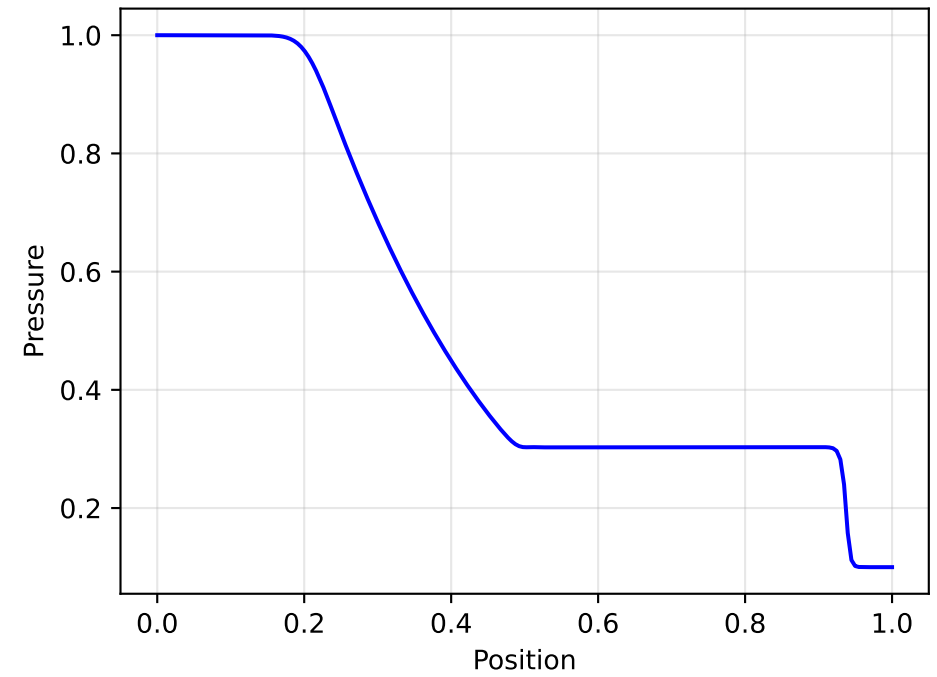
Sod Shock Tube: Pressure
