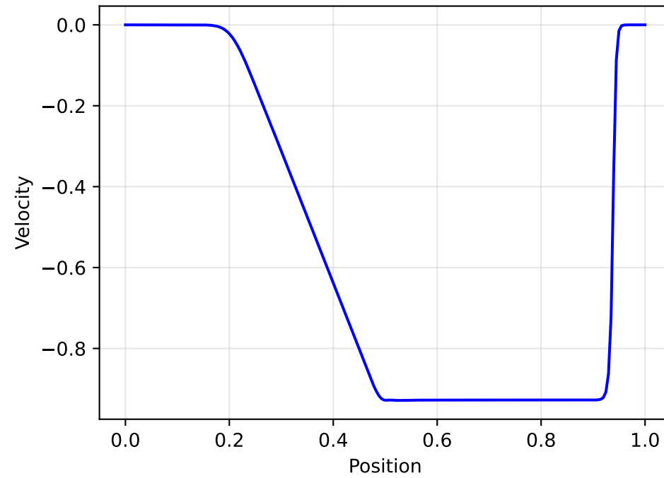
Sod Shock Tube: Velocity
