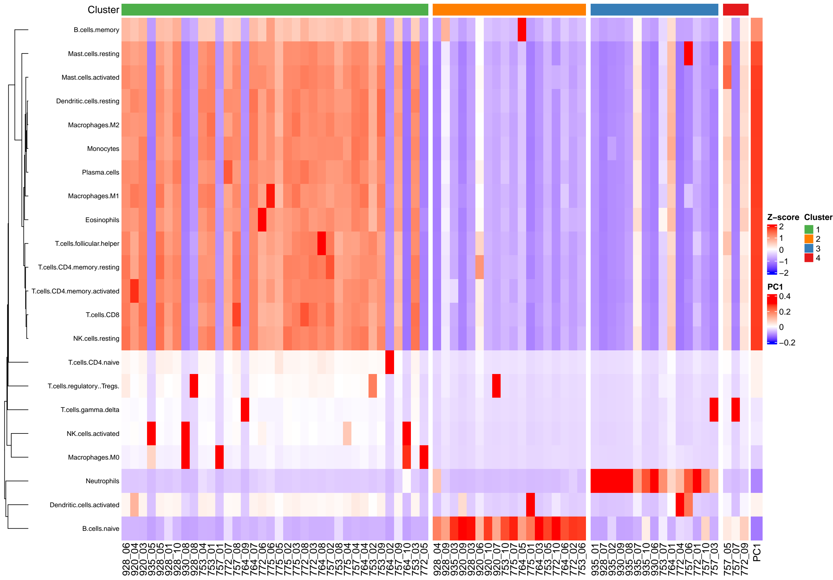
SD:skmeans, k = 4
