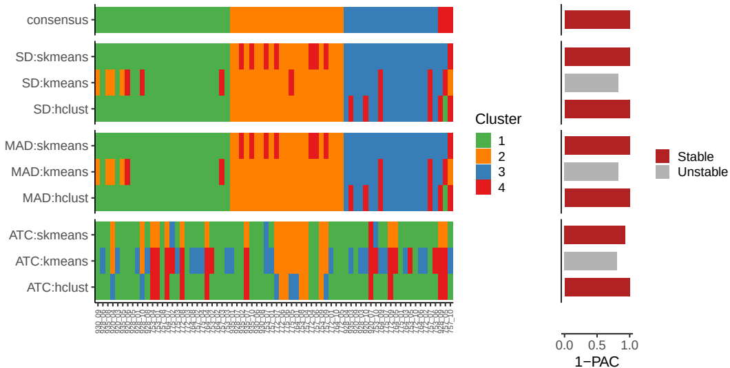
Classification from all methods, k = 4
