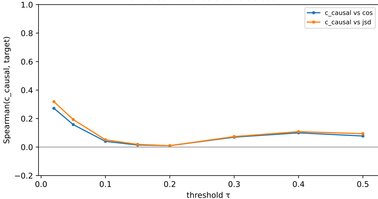
Is the coincidence stable across \tau ?
