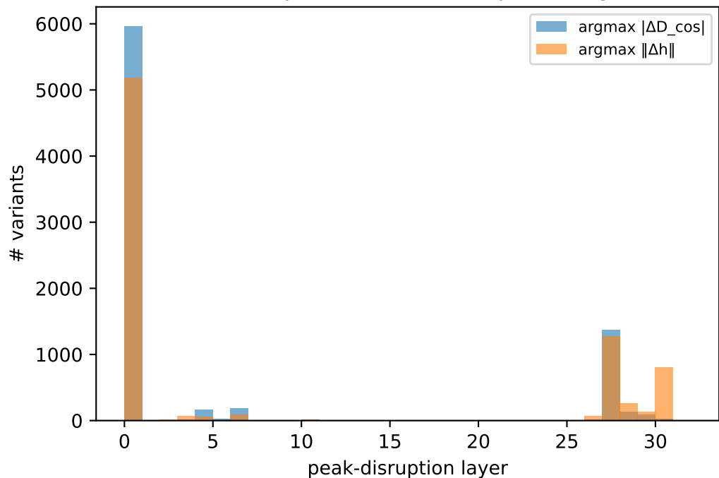
Localization: spread (cosine) vs spike (magnitude)
