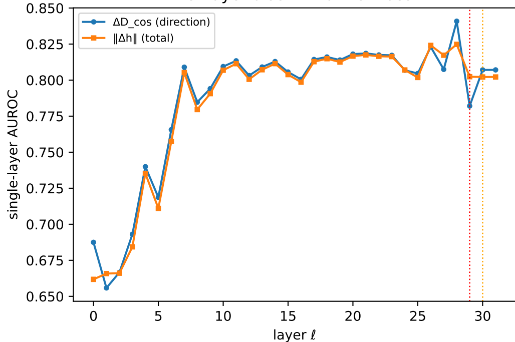
Per-layer discriminative mass
