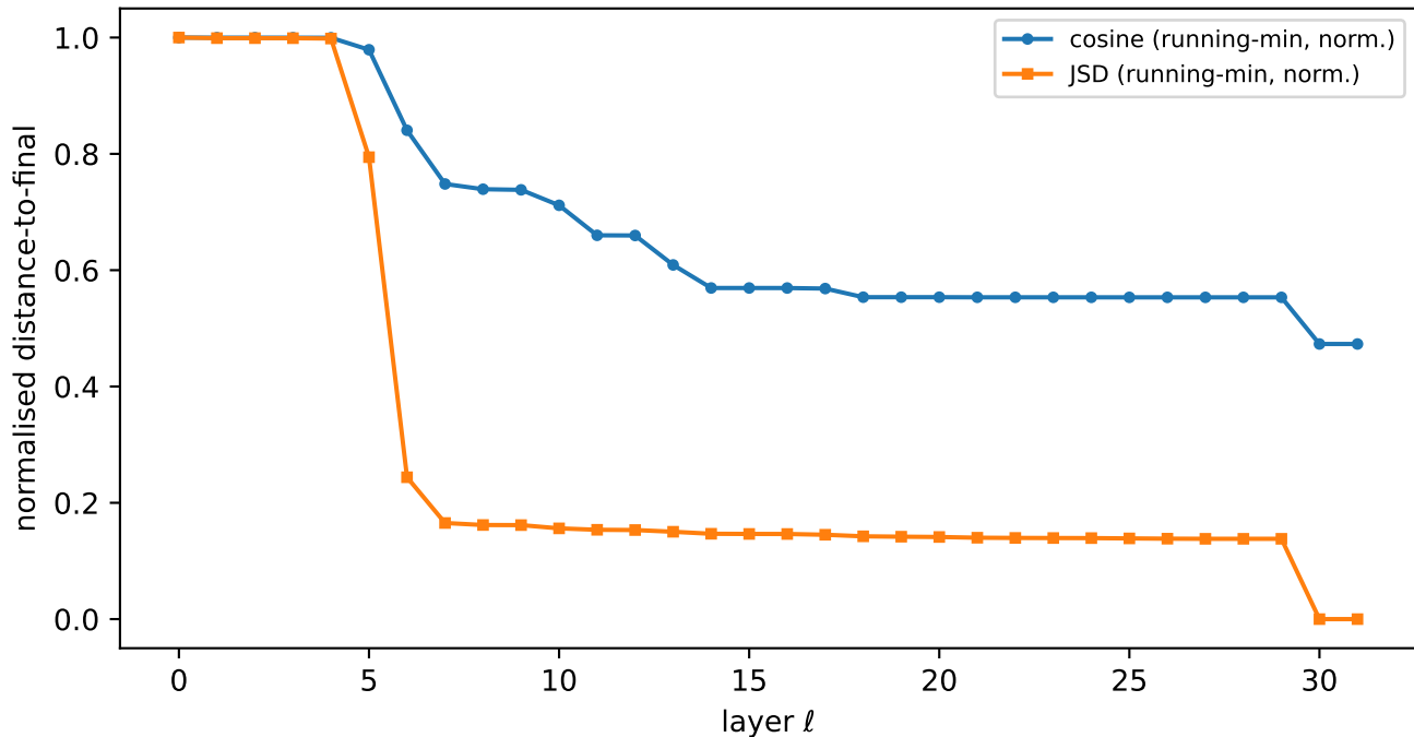
Cosine descends smoothly; JSD is a near-binary cliff
