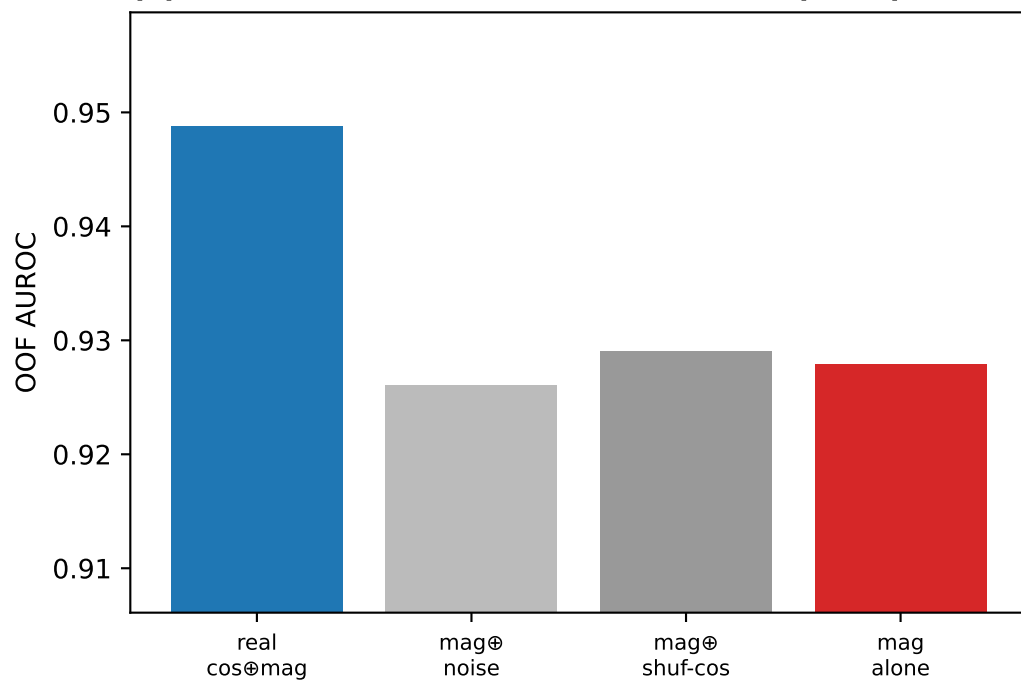
(c) H9c matched-dimension controls (64-d)
