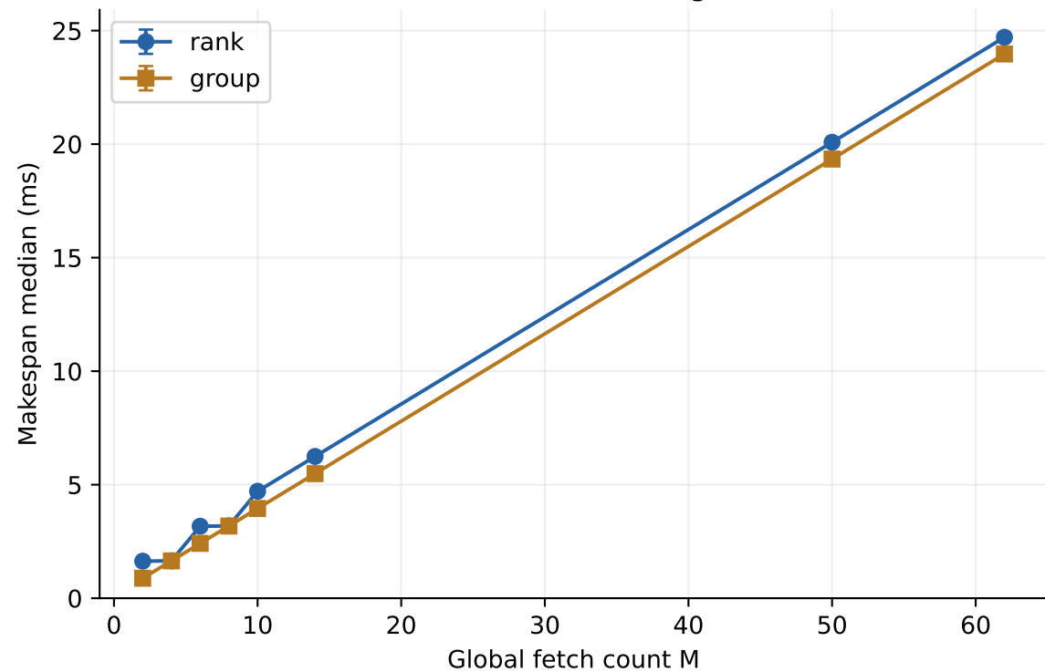
Miss-count scaling
