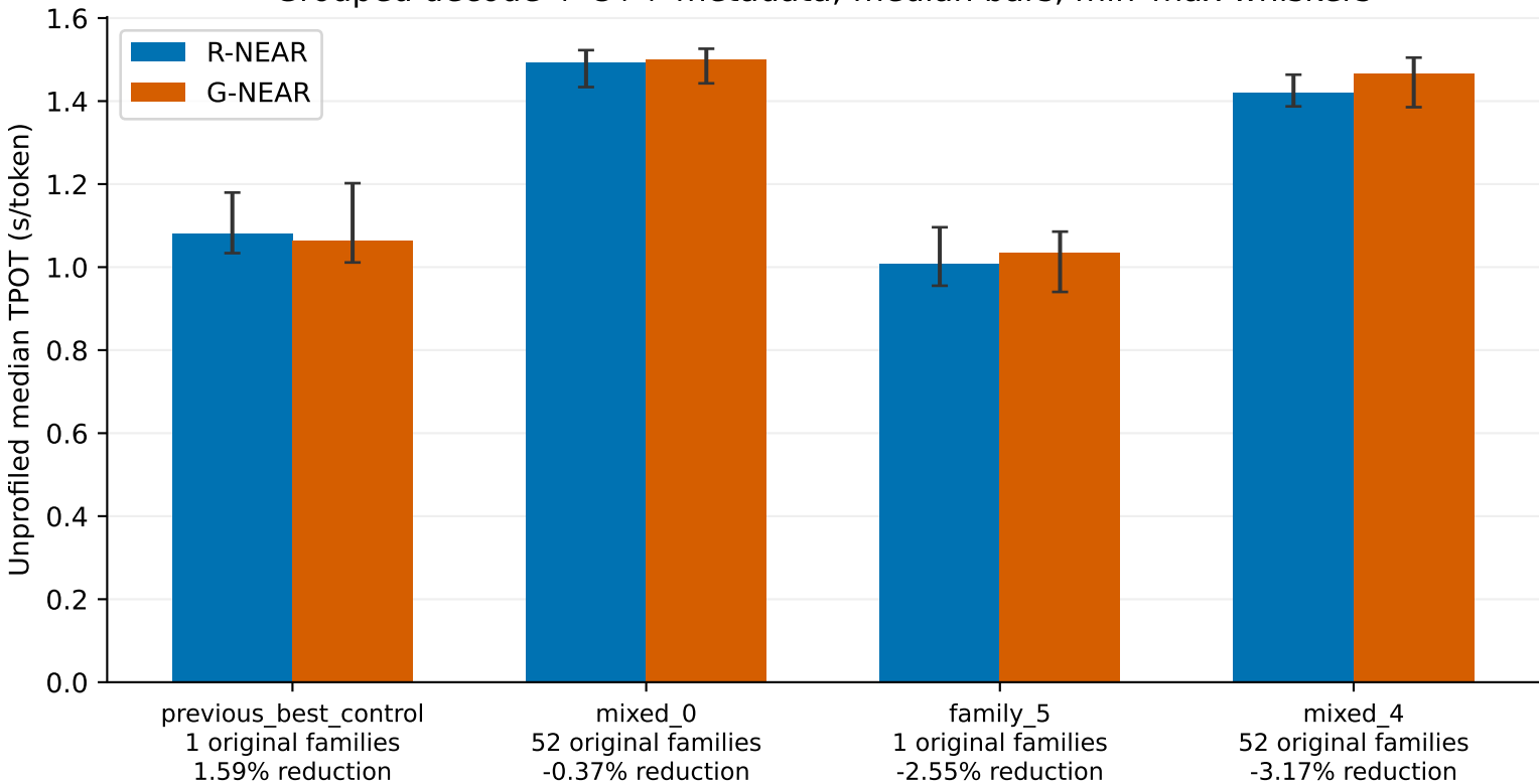
ShareGPT local B16, global 64, output 128: 4 finalists, 5 repeats/arm Grouped decode + C++ metadata; median bars, min-max whiskers
