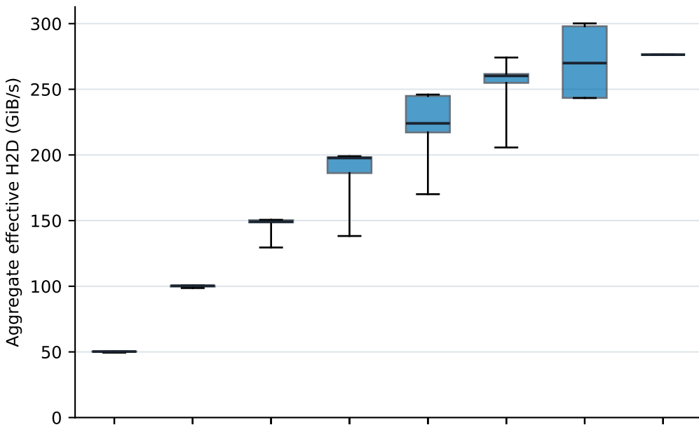
DeepSeek expert · aggregate
