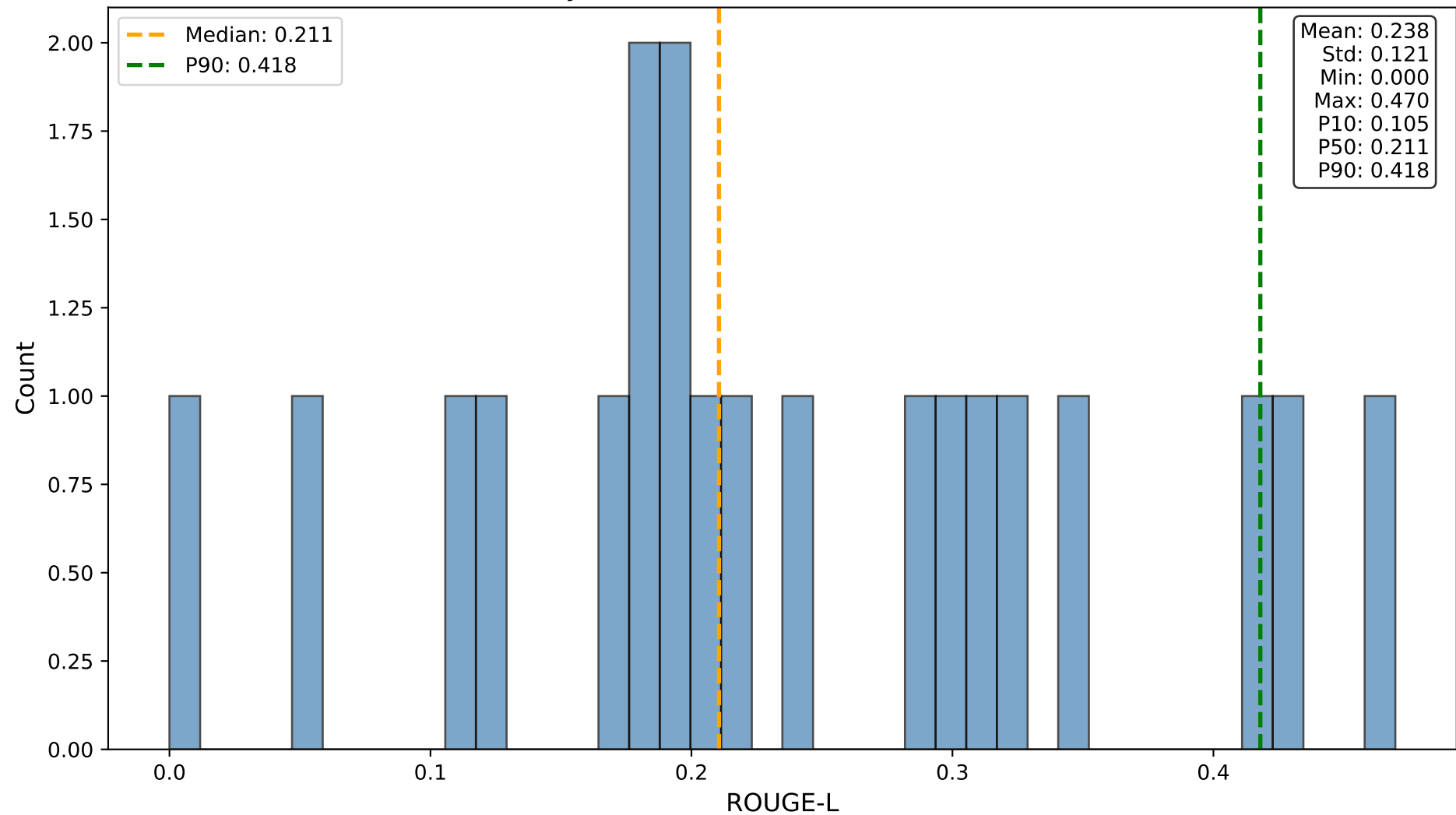
Z-only Generation ROUGE-L Distribution
