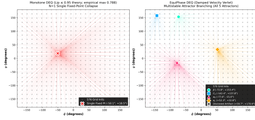
Figure 3: Verified Banach contraction (theoretical bound 0.95; empirical Lipschitz max 0.788):
