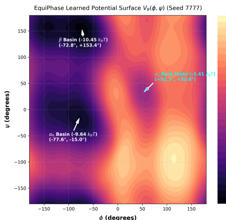
Figure 2: Learned potential V_\theta(\phi, \psi) , seed 7777. Basin minima and their depths, restated here for print legibility: \beta basin at (-72.8^\circ, +153.4^\circ) with V(\beta) = -10.45 kBT; \alpha R basin at (-77.6^\circ, -15.0^\circ) with V(\alpha R) = -9.64 kBT; hence \Delta F = +0.81 kBT with the correct ordering V(\beta) < V(\alpha R) .
