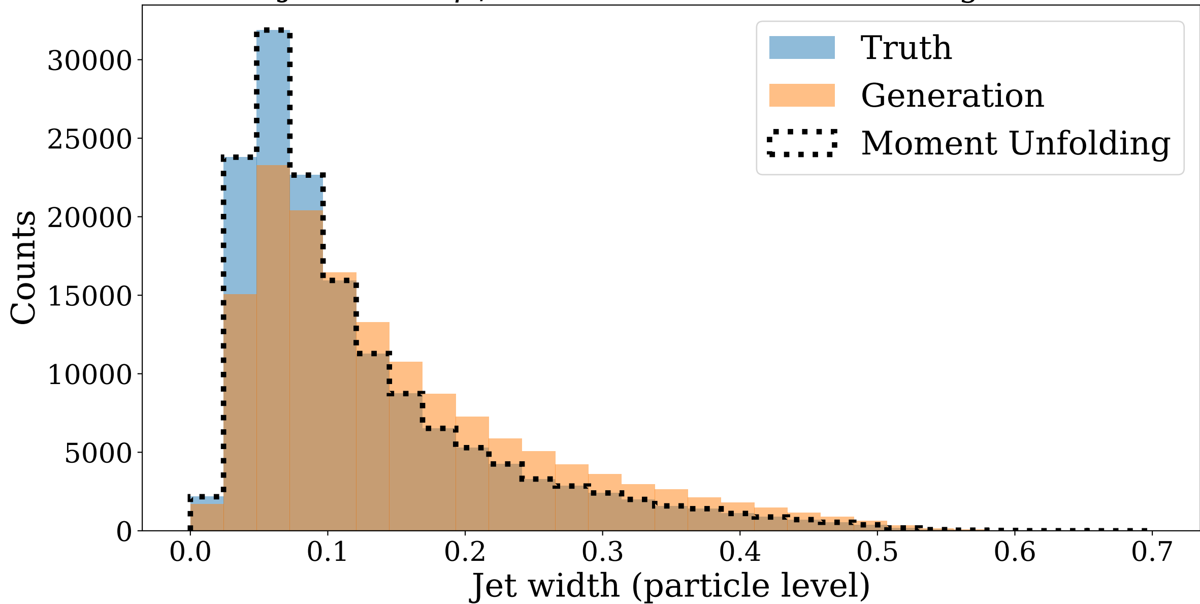
Jet Width: p_T Conditioned Inclusive Histograms
