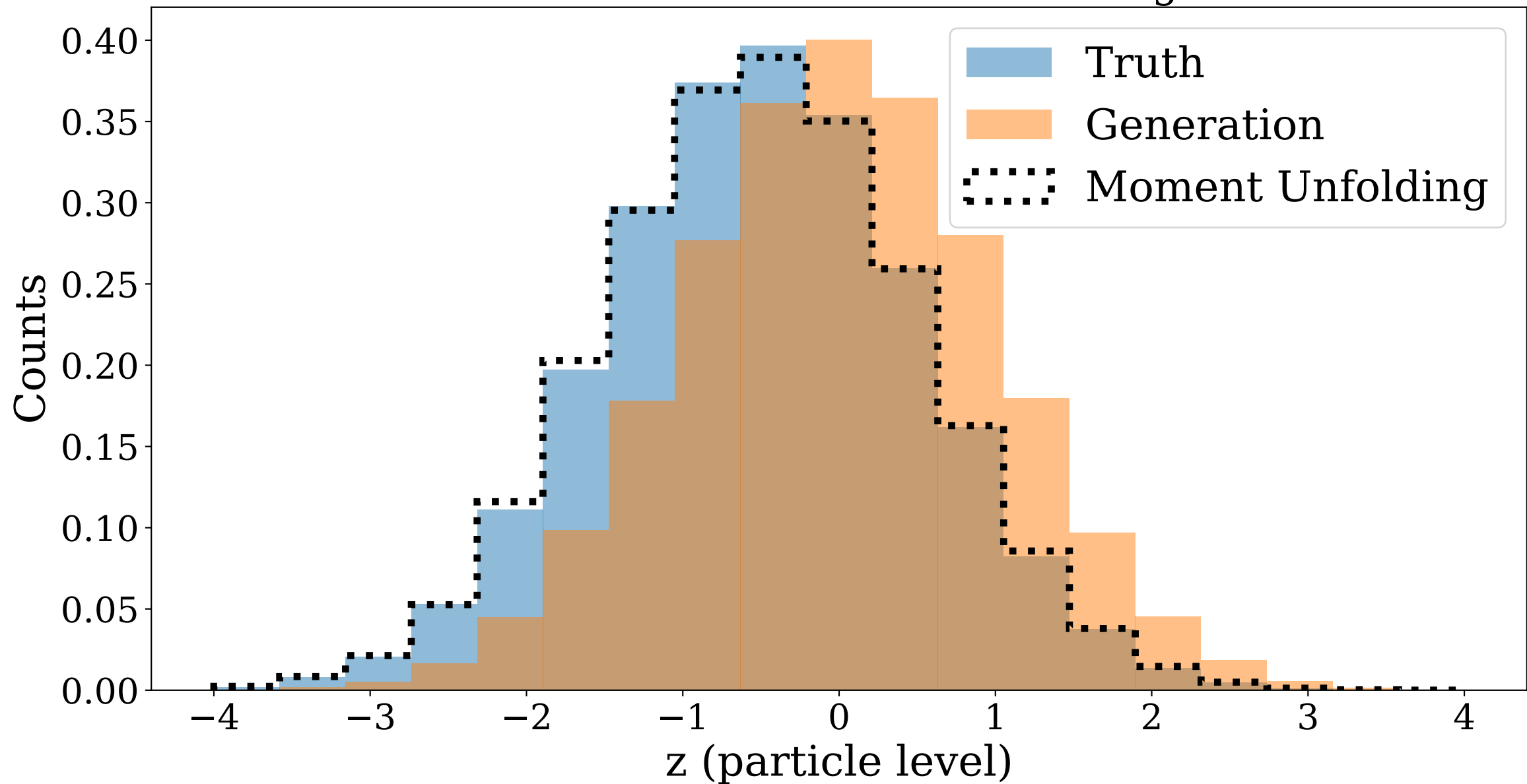
Gaussian Data: Particle Level Histograms
