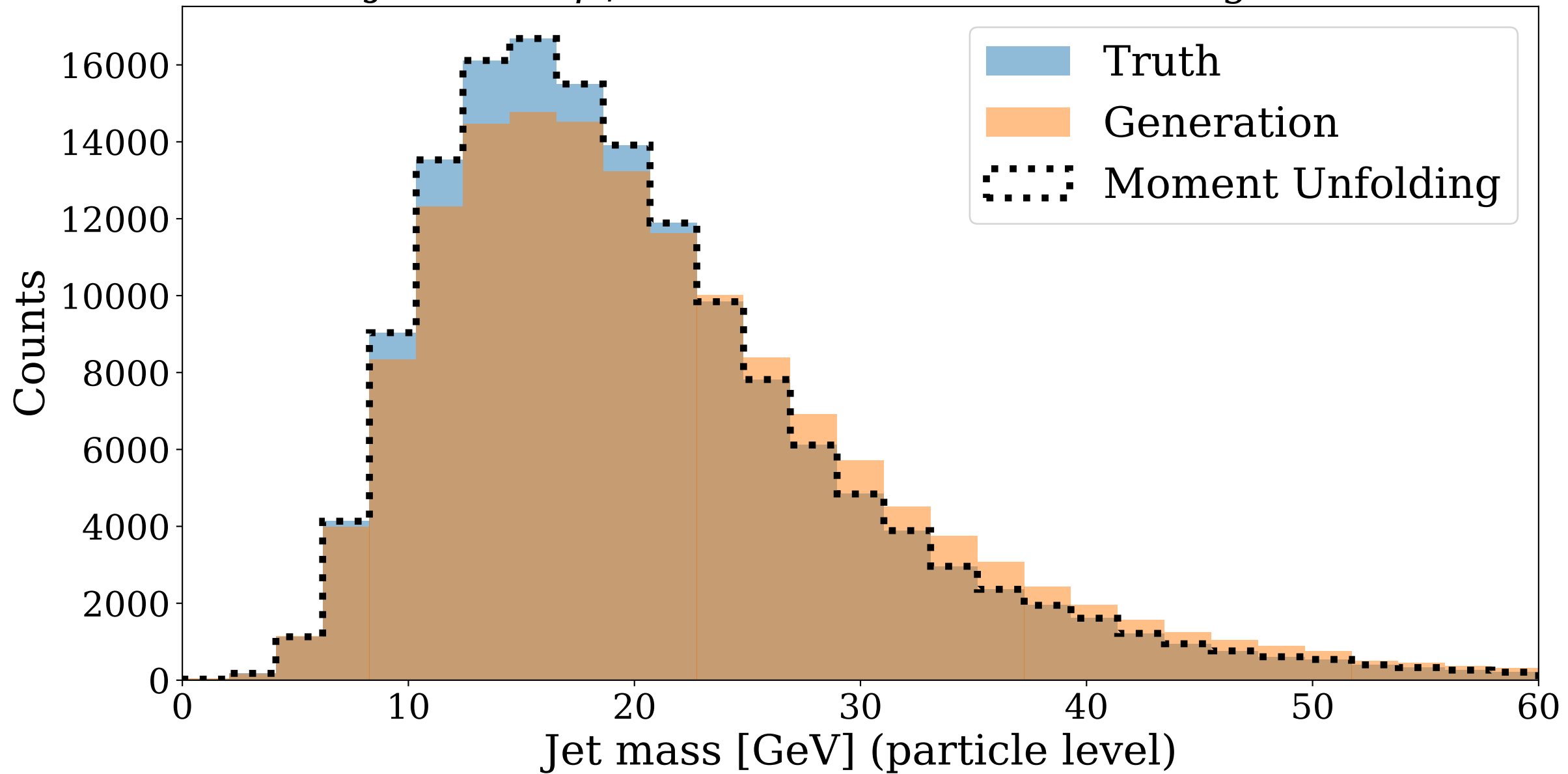
Jet Mass: p_T Conditioned Inclusive Histograms
