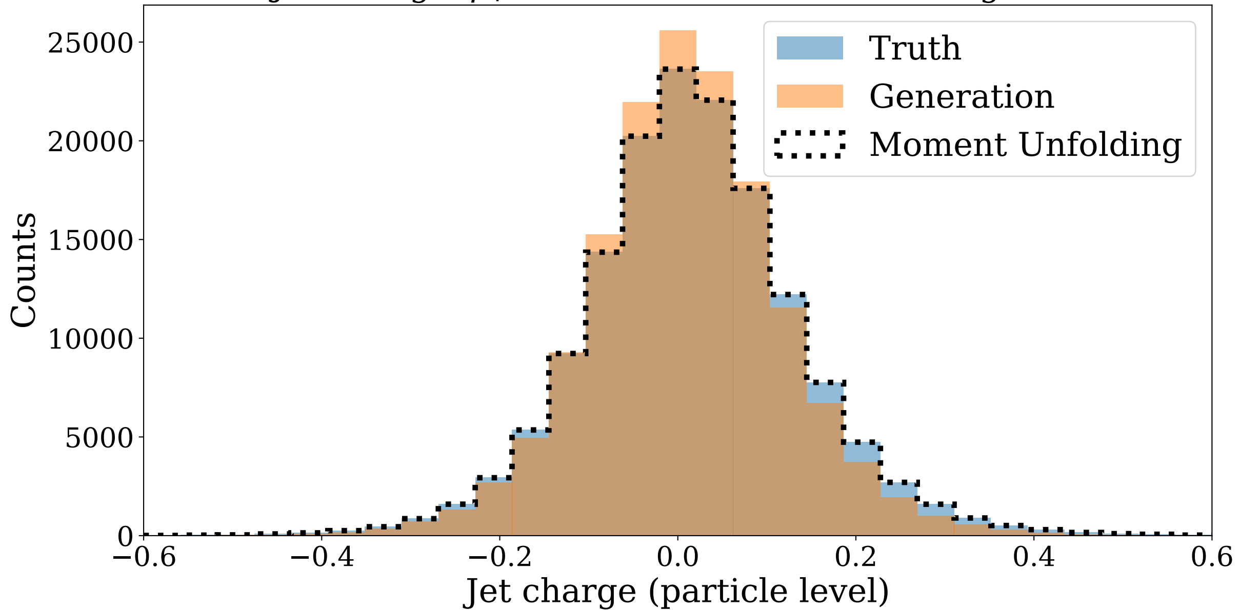
Jet Charge: p_T Conditioned Inclusive Histograms
