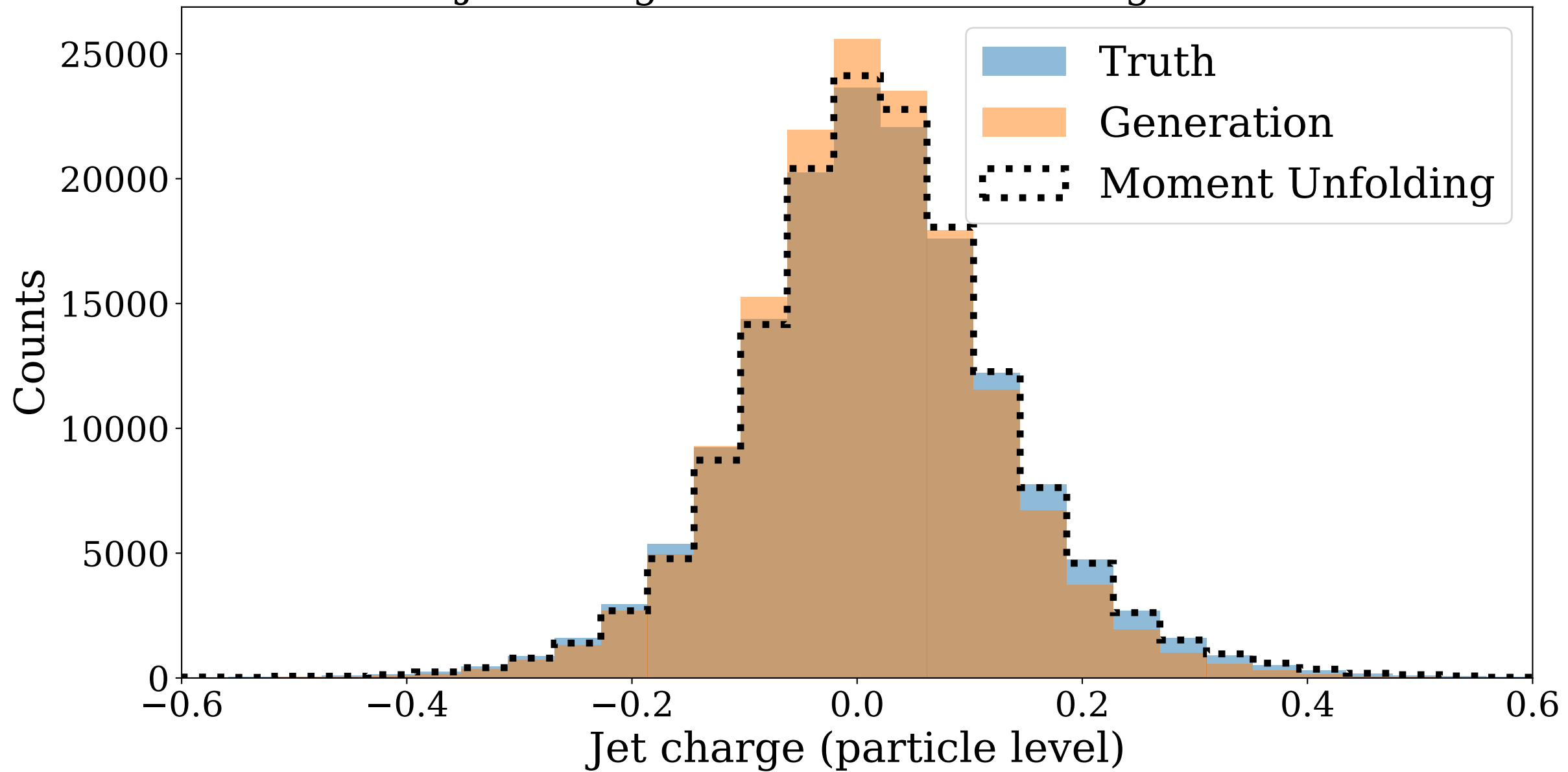
Jet Charge: Particle Level Histograms
