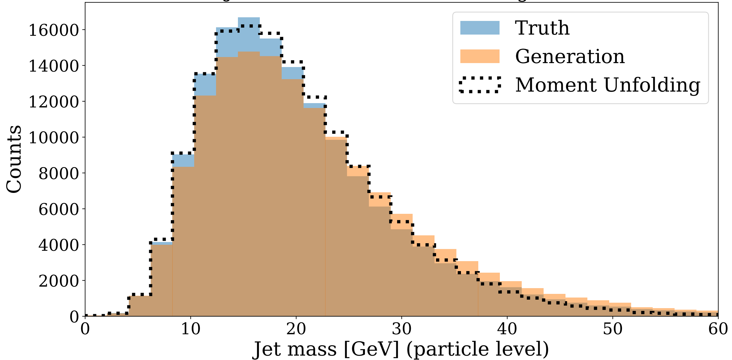
Jet Mass: Particle Level Histograms
