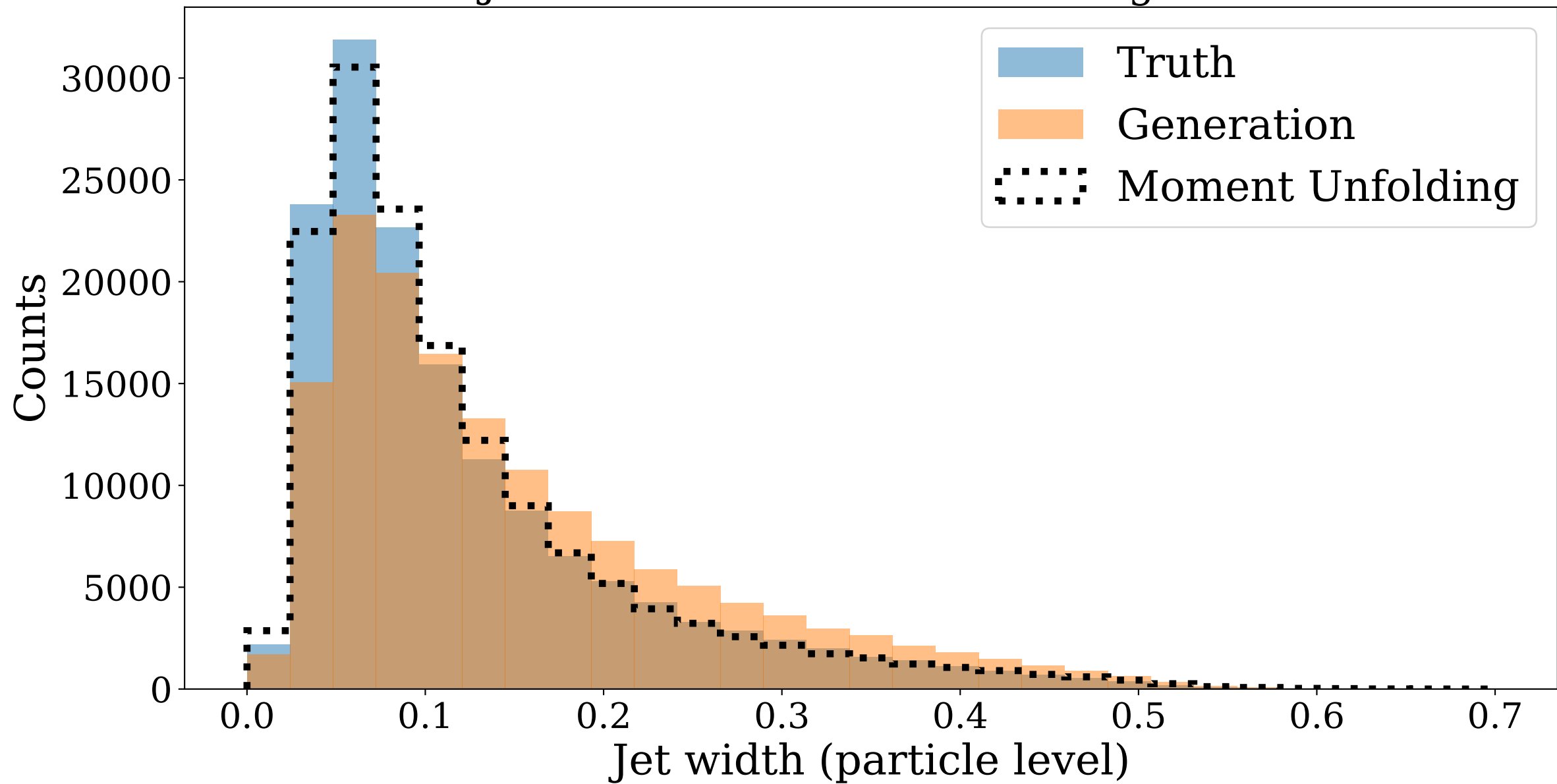
Jet Width: Particle Level Histograms
