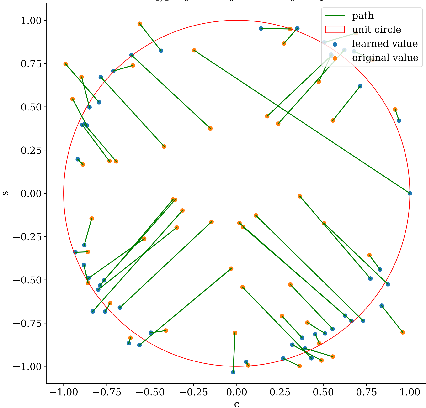
N_{1,1} : Symmetry Discovery Map
