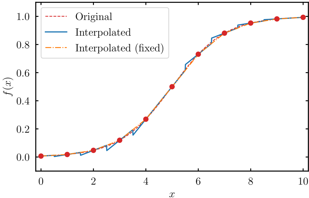
Linear interpolation ( x in increasing order)
