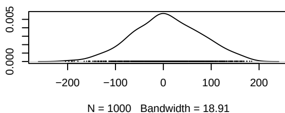
Density of idegree1
