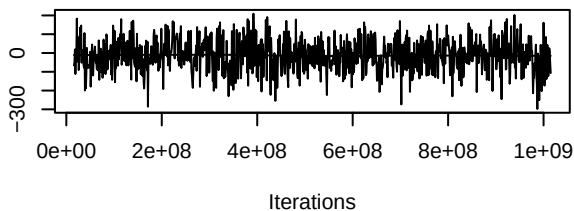
Trace of dnf.chicago.1.f
