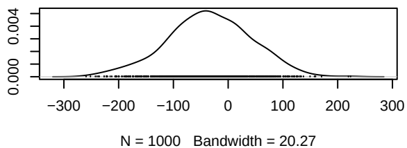
Density of dnf.chicago.2.n
