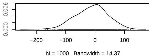
Density of mix.race.num.2.2
