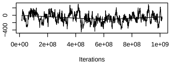
Trace of dnf.chicago.1.n
