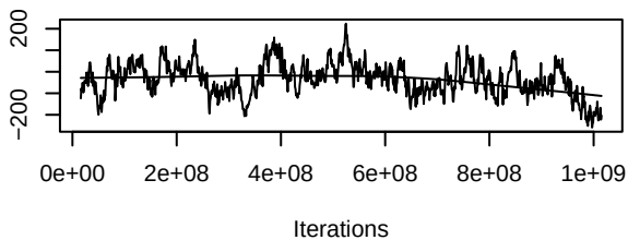
Trace of dnf.chicago.2.n
