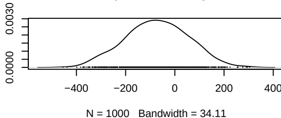
Density of dnf.chicago.1.n
