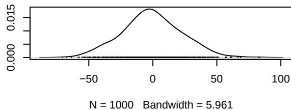
Density of mix.race.num.4.1
