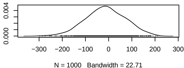
Density of dnf.chicago.1.f
