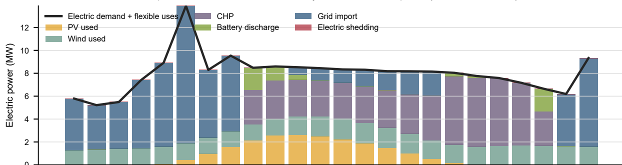
Representative shoulder-season day: deterministic dispatch (2019-05-02, UTC)
