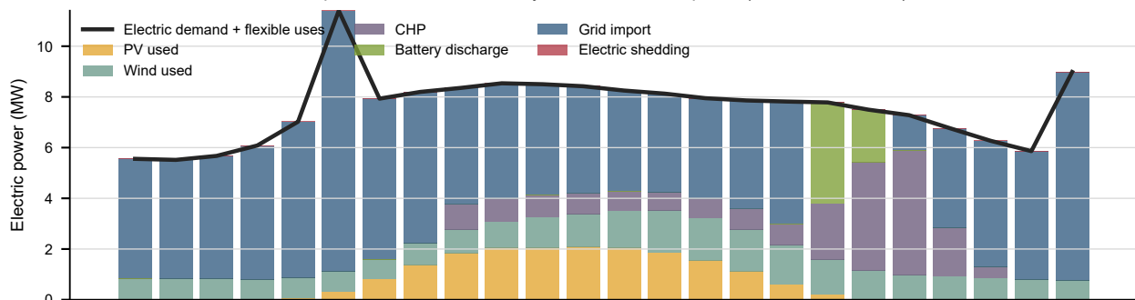
Representative summer day: deterministic dispatch (2018-08-14, UTC)
