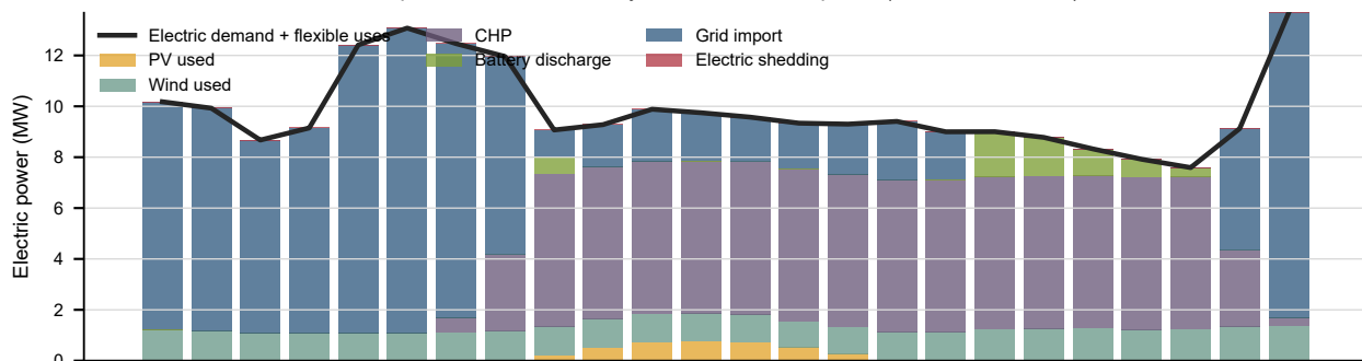
Representative winter day: deterministic dispatch (2018-01-19, UTC)
