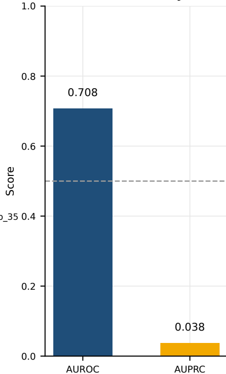
c Global hard-safety detection
