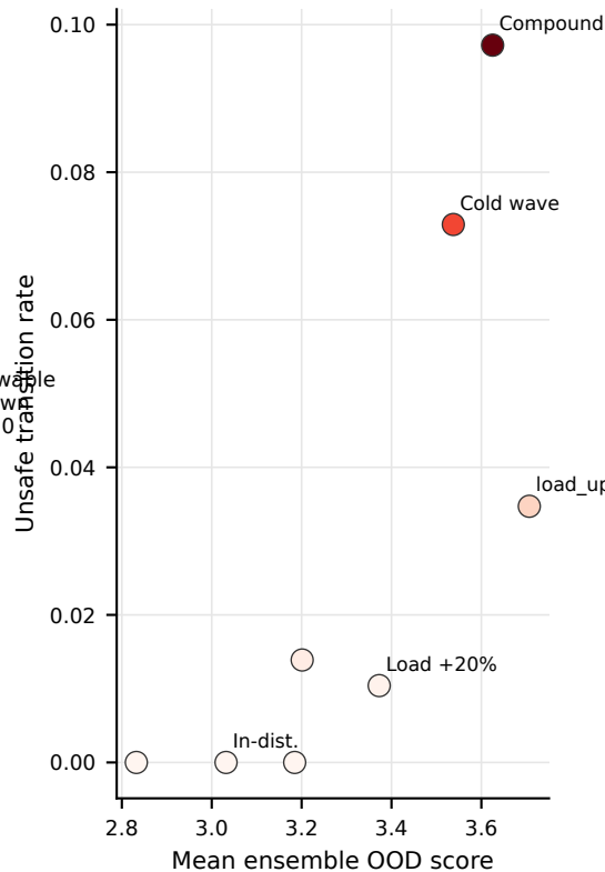
b Risk is useful but imperfect
