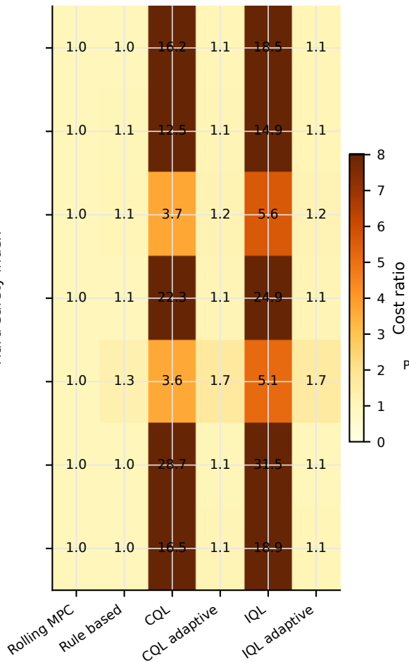
b Cost relative to rolling MPC
