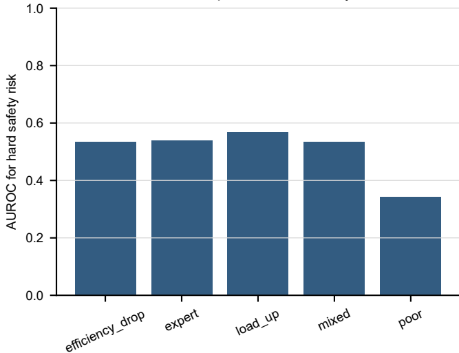
OOD score predicts hard-safety risk
