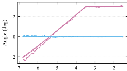
(a) Solar-Cells; 0.5 mm/s; Pitch sweep
