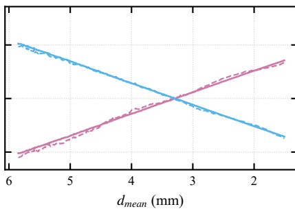
(i) OSRs; 0.9 mm/s; Diagonal opposite
