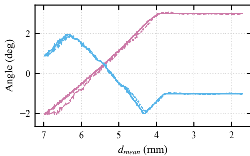
(g) OSRs; 0.5 mm/s; Pitch-roll coupled
