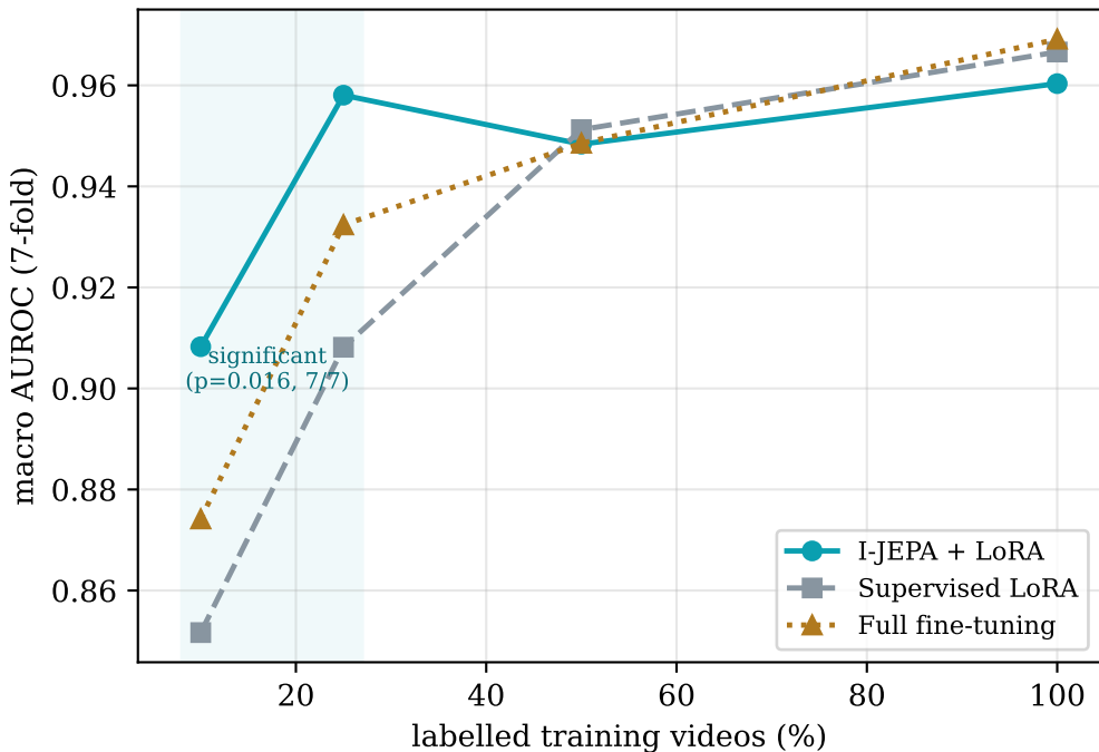
Label efficiency: I-JEPA wins when labels are scarce
