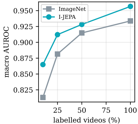
(c) Label efficiency
