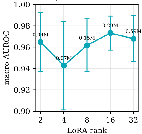
(b) Rank ablation
