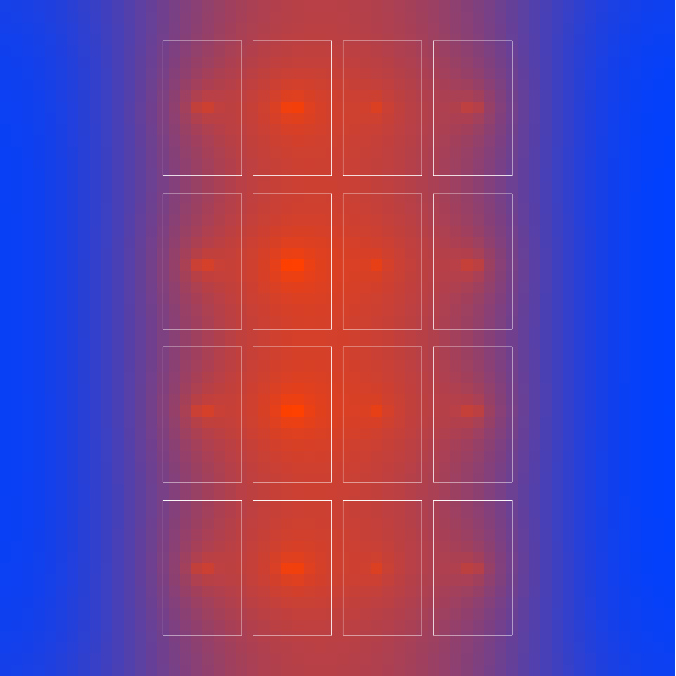
T min 55.3 °C (blue) ... max 64.3 °C (red); ambient 45 °C; B-gated-drain
