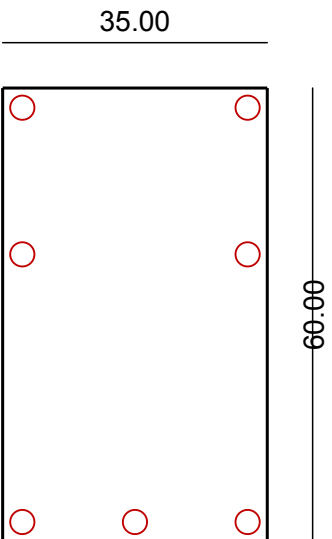
RF Power Amplifier — 35.0 × 60.0 mm, 7 holes/mounting pads source RF_PA.brd (EAGLE 9.6.2)
