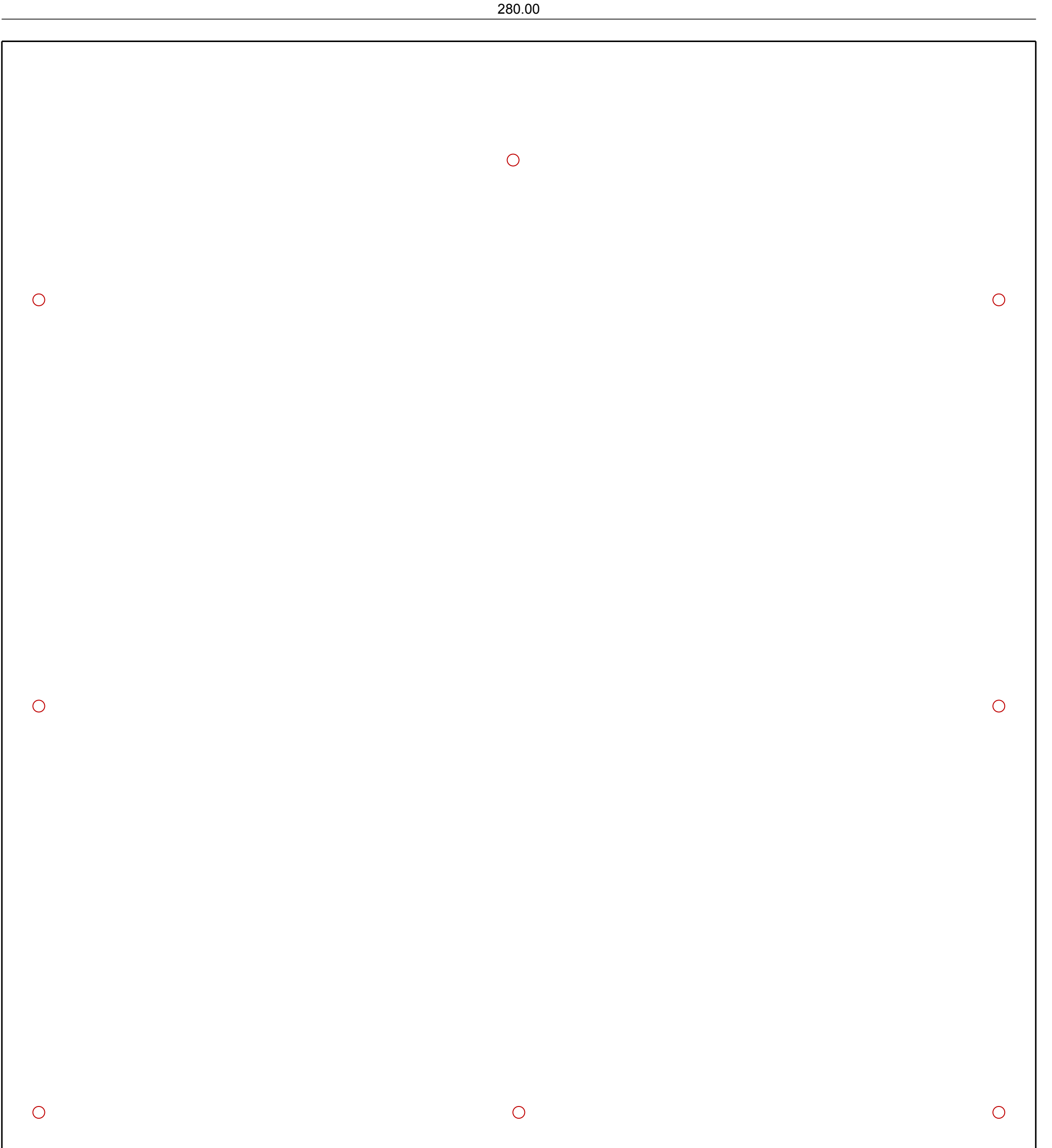
Power Supply Board — 280.0 × 300.0 mm, 8 holes/mounting pads source PowerBoard.brd (EAGLE 7.4.0)
