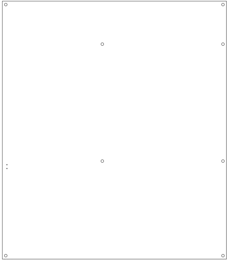
Drill Map: x 0.900mm / 0.0354" (2 holes) (not plated) O 3.200mm / 0.1260" (8 holes) (not plated)
