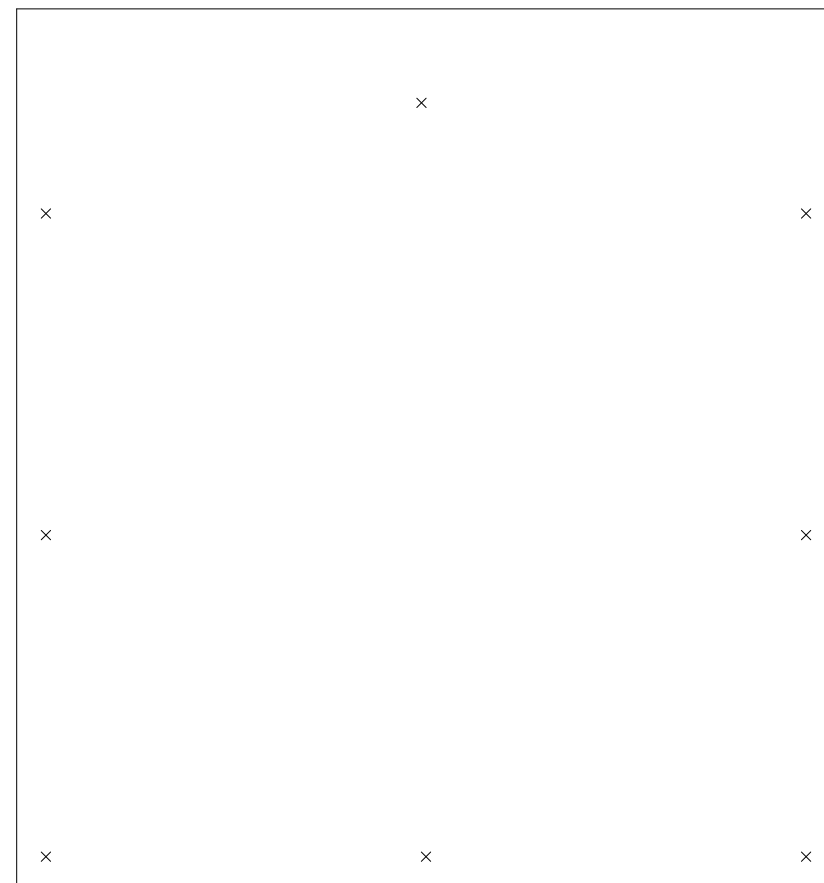
Drill Map: x 3.200mm / 0.1260" (8 holes) (not plated)
