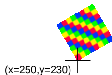
Rotating image
