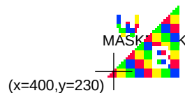
masked image
