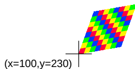
Skewing image
