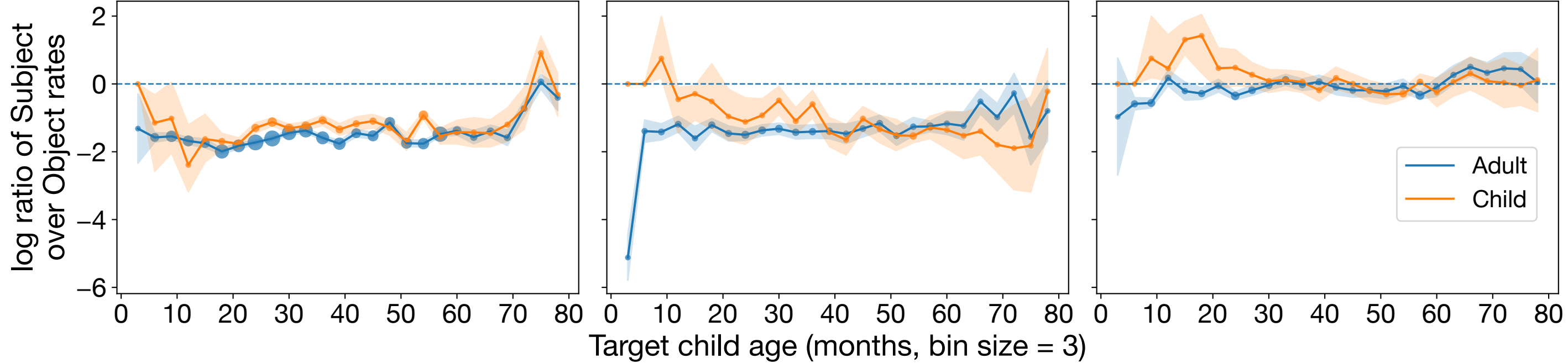
Matrix Questions
