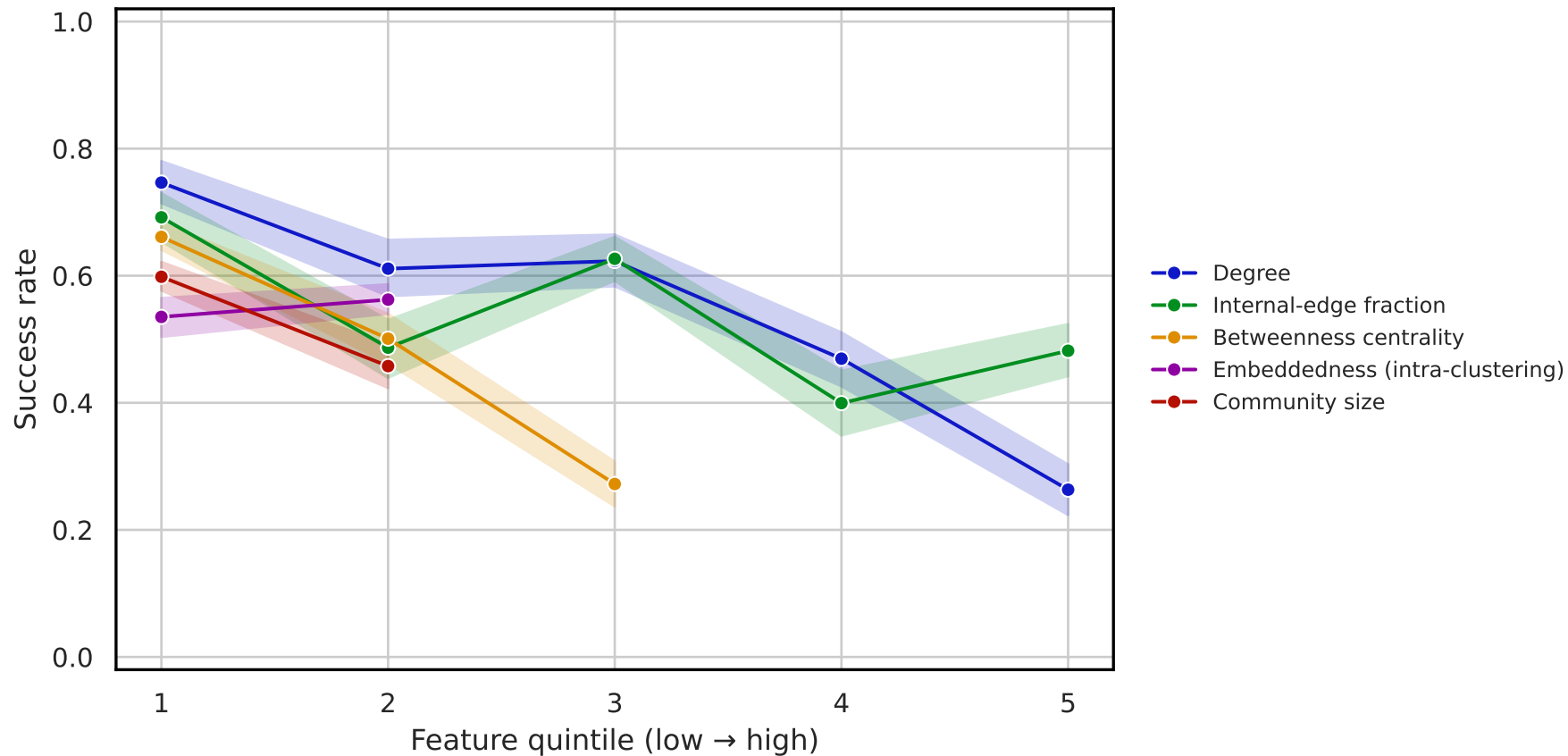
cond-mat — dgcluster — \nabla -CMH
