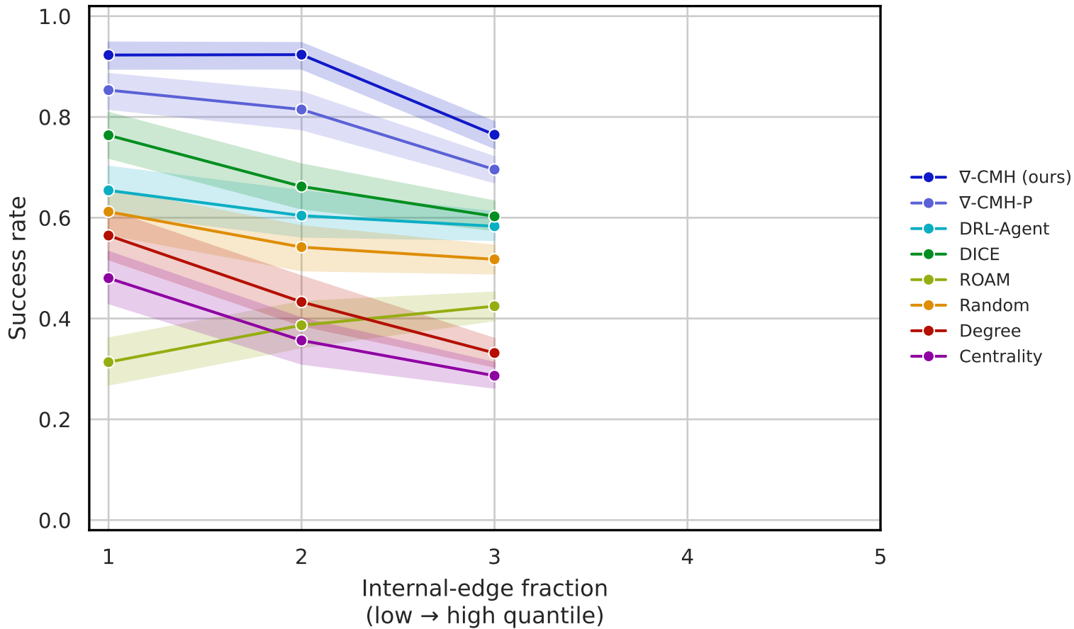
vote — greedy
