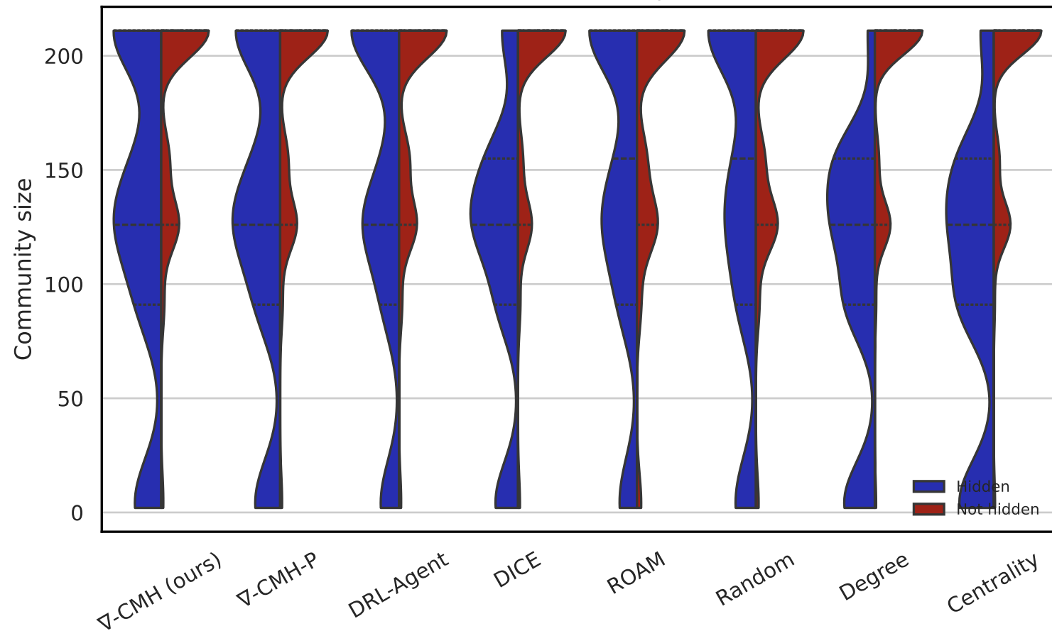
vote — walktrap
