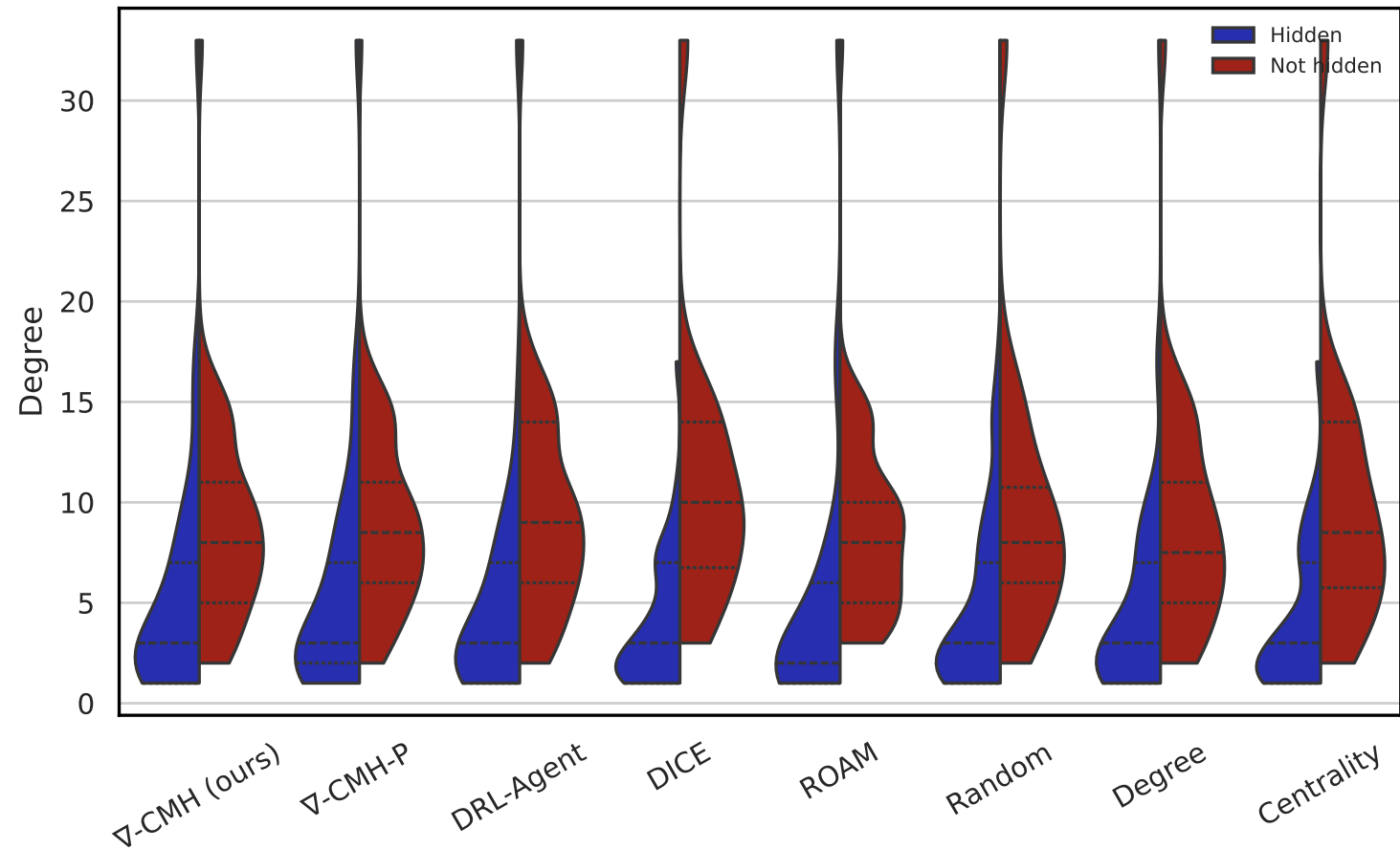
words — walktrap
