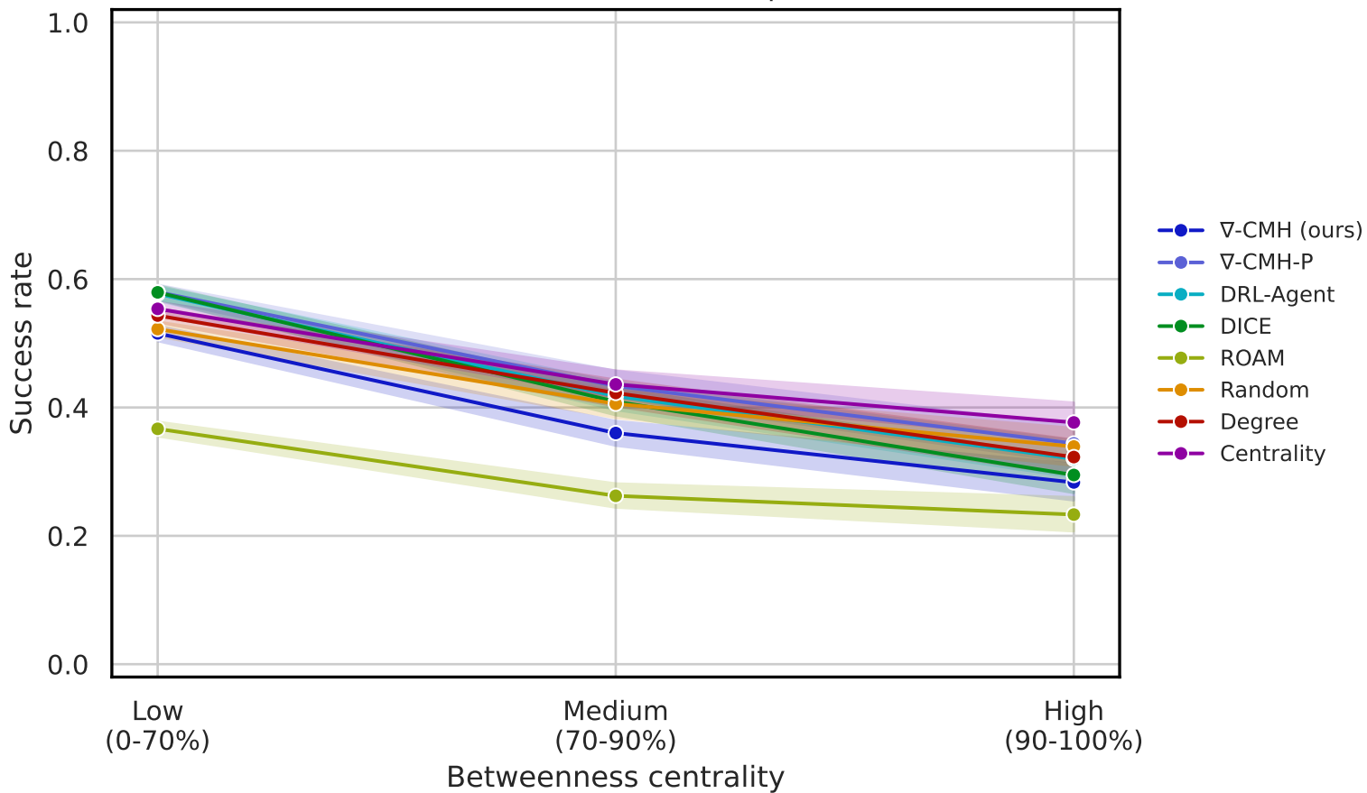
all datasets — walktrap
