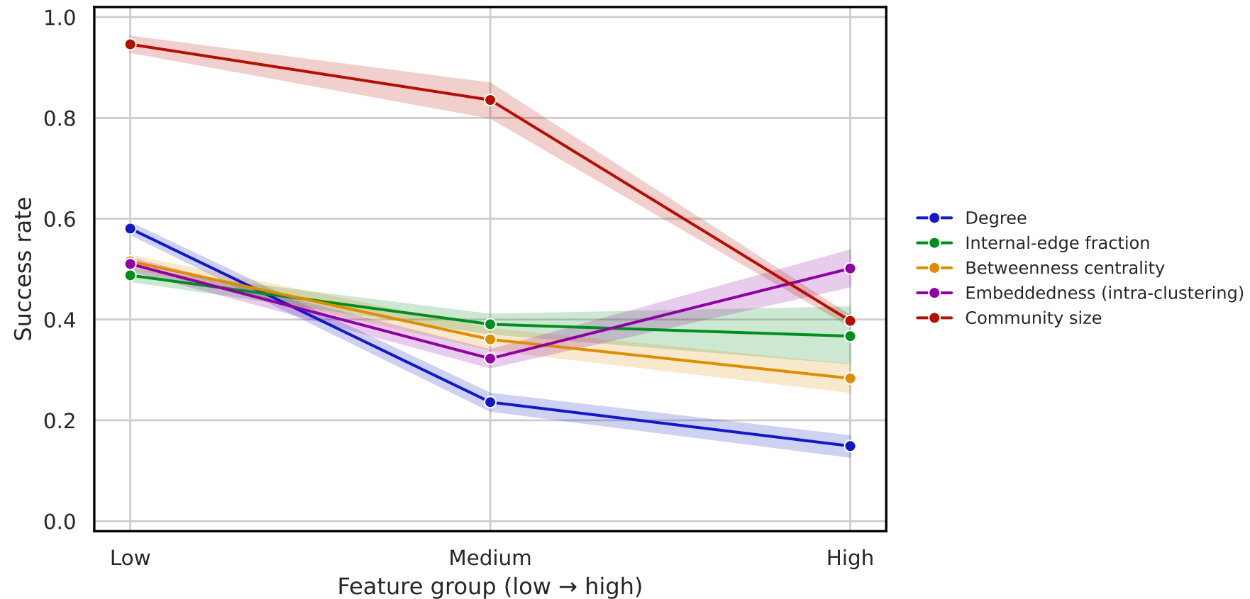
all datasets — walktrap — \nabla -CMH
